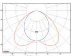
LED MALL LINE 70 D120 IP54 4000K
